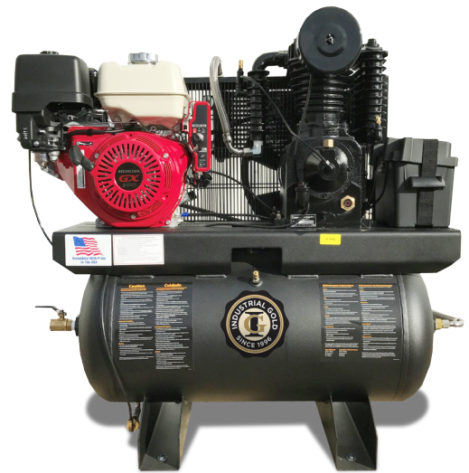
Air cooled after cooler Platinum unit
