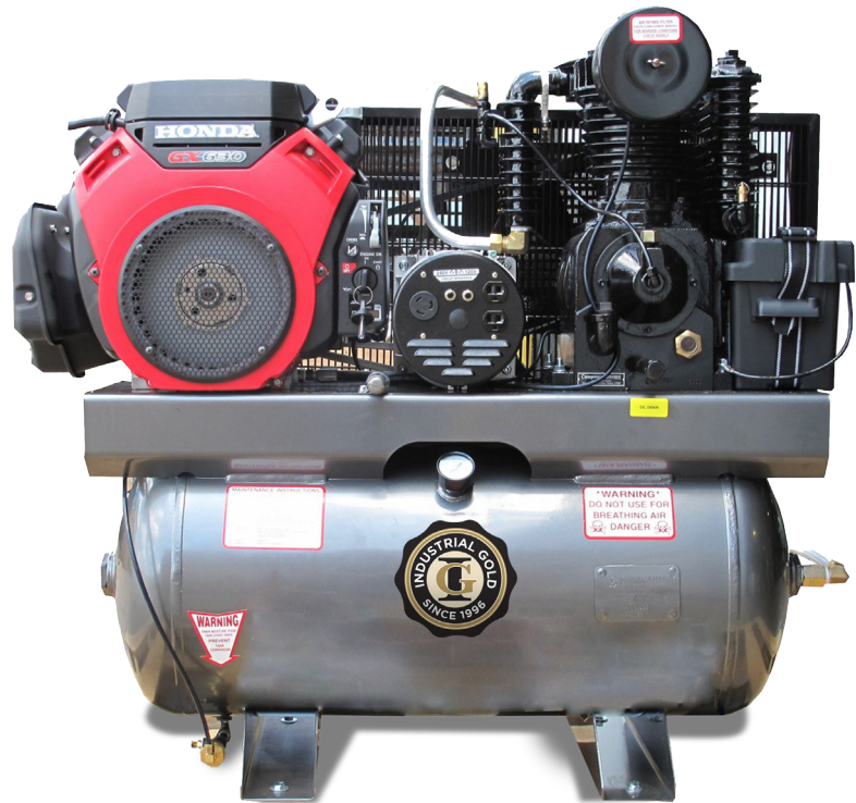
Air cooled after cooler Platinum unit
